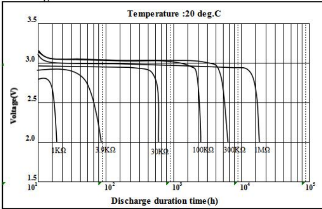
Discharge Characteristics
